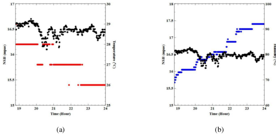
Figure 3. (a) The graph of NSB and temperature versus time on March, 9 th 2018 on constant NSB. (b) The graph of NSB and humidity versus time on March, 9 th 2018 on constant NSB.
