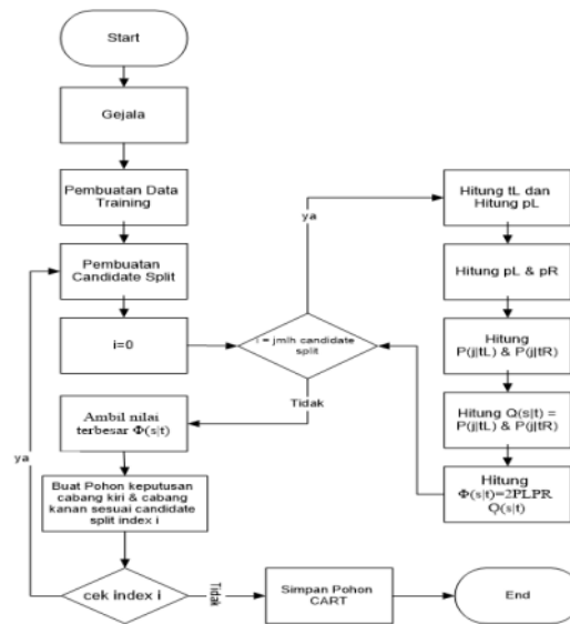
Gambar 3 Flowchart metode CART
