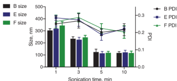
Figure 5. Size (columns) and PDI (lines) of w/o emulsion produced from formulations B (black), E (blue) and F (green) obtained after 1–10 min of HES exposure. Samples were emulsified using the same energy settings.
