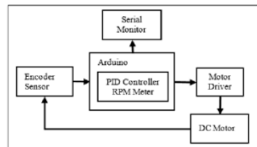
13 Fig. 1. The Block Diagram System
