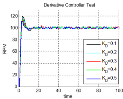
Fig. 7. The system's response of Derivative control
