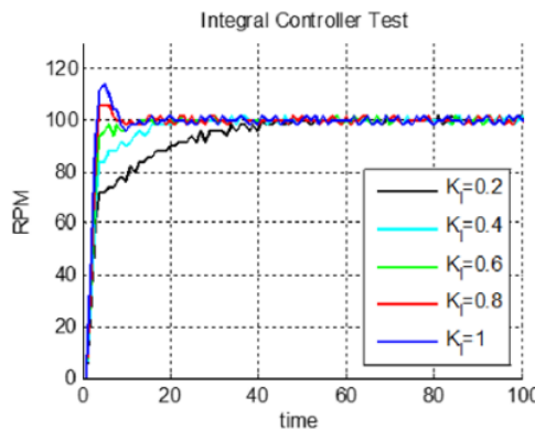
Fig. 6. The system's response of Integral control
