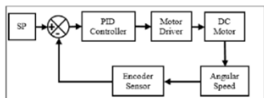
Fig. 2. The Control System Block Diagram
