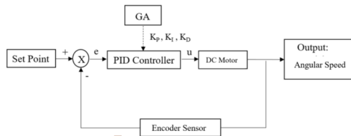
Fig. 1. PID controller tuning block diagram
