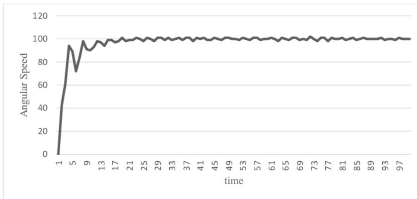
Fig. 26. Graph GA crossover 0.4 Method on Hardware Testing
