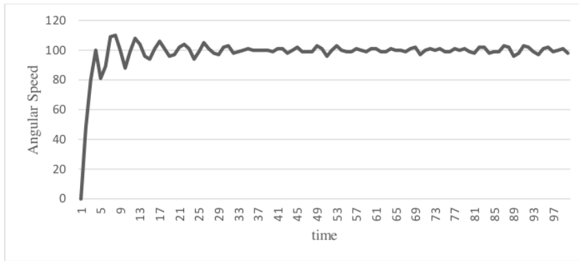
Fig. 25. Graph GA crossover 0.2 method on Hardware Testing
