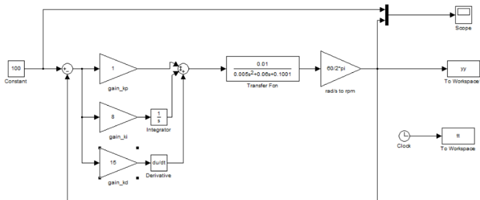
Fig. 5. DC Motor Plant at Matlab
