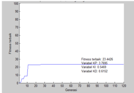
Fig. 16. The Fitness Results Number of Generations 120
