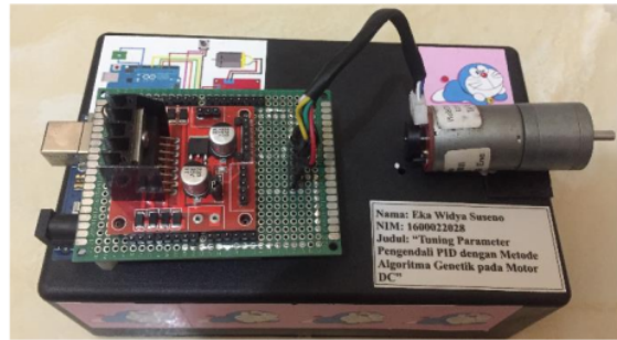
Fig. 20. PID Control Hardware with DC Motor
