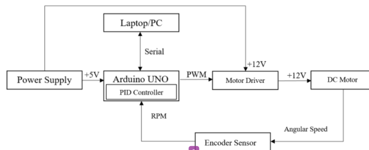
Fig. 2. Hardware Block Diagram
