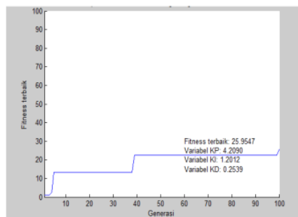
Fig. 13. The fitness and PID parameter results with the crossover constant are 0.4
