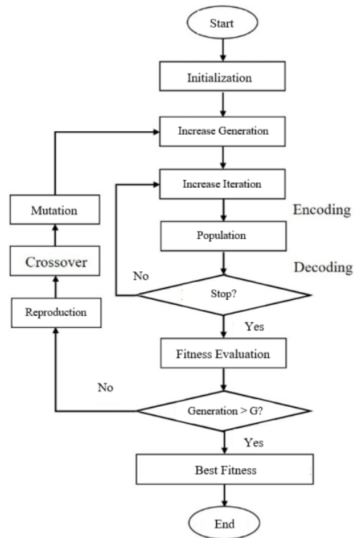
Fig. 4. Genetic algorithm program flowchart
