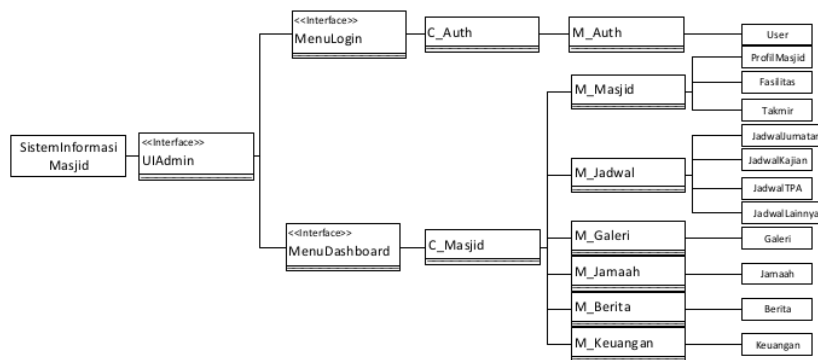
Gambar 6. Class Diagram View Admin
