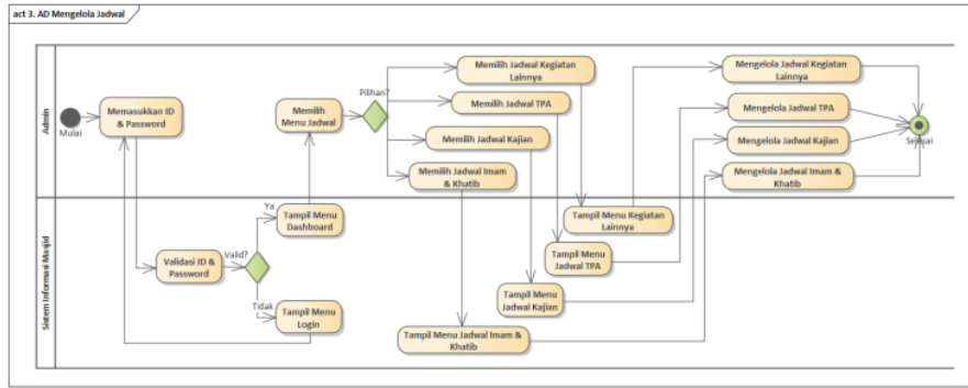
Gambar 5. Activity Diagram Mengelola Jadwal
