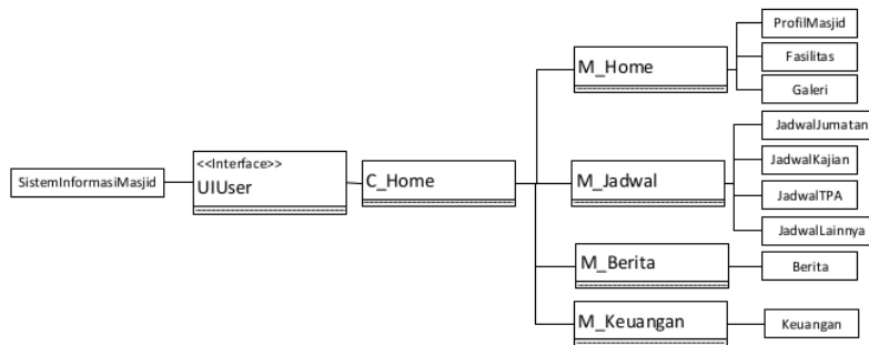
Gambar 7. Class Diagram View User
