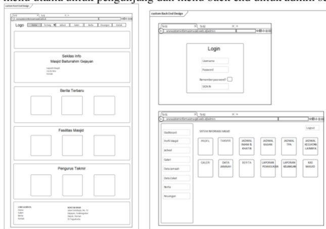
Gambar 9. Desain User Interface
