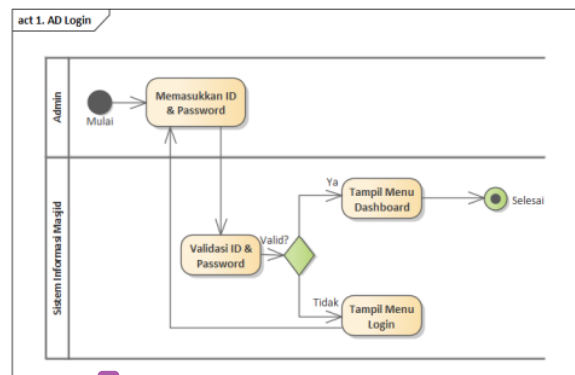
Gambar 4. Activity Diagram Login Admin
