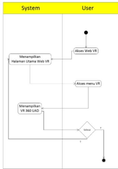
Gambar 6. Proses Bisnis
