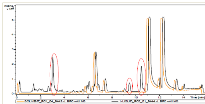
Fig. 4: LC-TOF-MS chromatogram of CM fraction, the oval circle shows the peaks of the compound contained in the CM fraction
