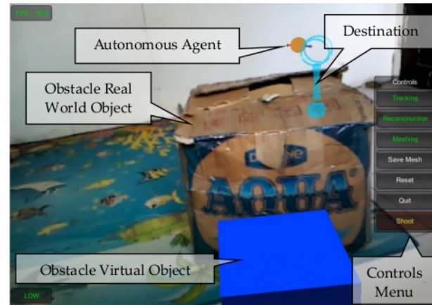
Fig. 5. User Interface with hidden mesh grid
