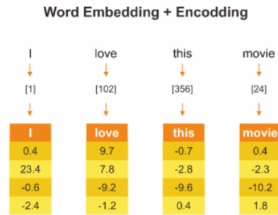
Figure 4. Word Embedding
