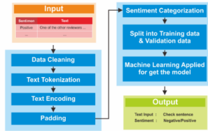
Figure 2. Machine Learning Approach for Sentiment Analysis
