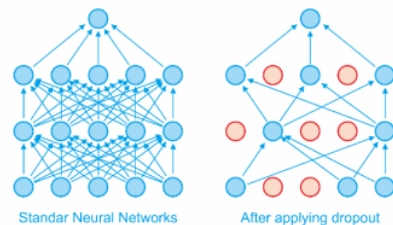
Figure 5. Dropout
