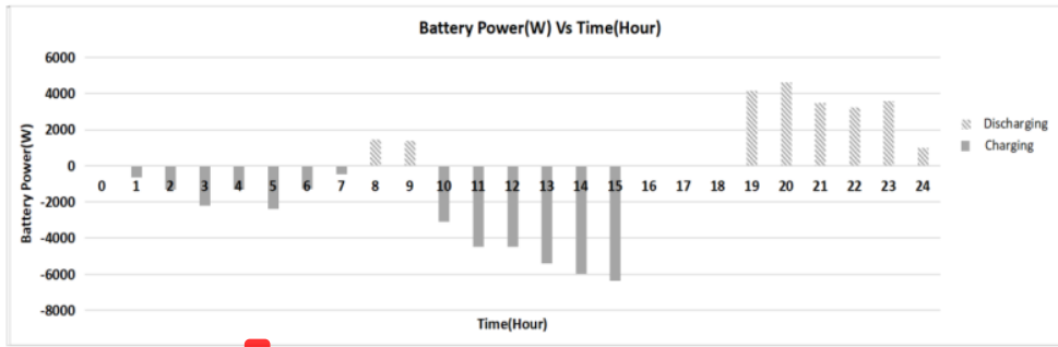
Figure 7. Battery Power on charging and discharging modes at the micro-grid
