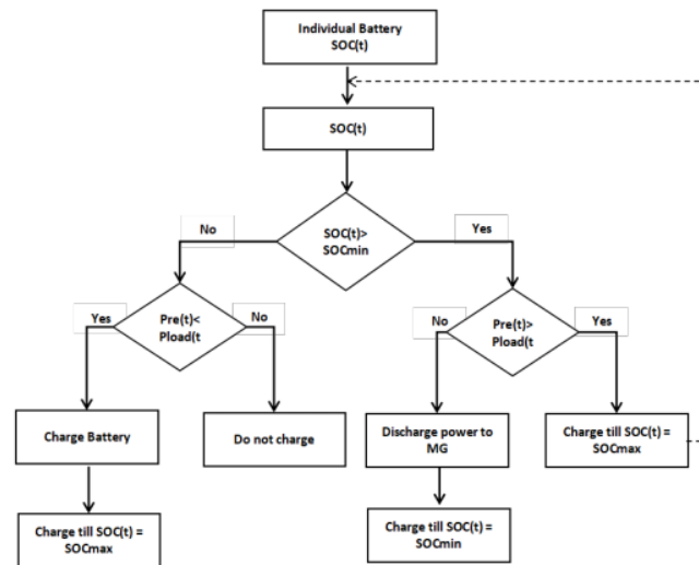
Figure 2. Flowchart of the Proposed M-G
