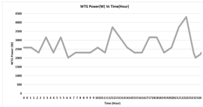
Figure 4. Power generation by wind turbine
