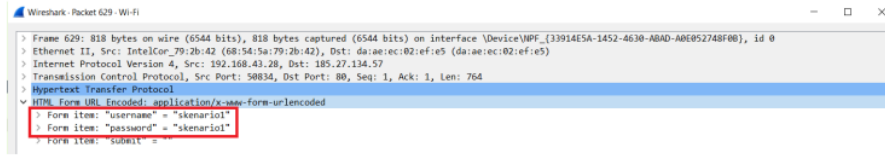
Figure 6. File Showing User Data
