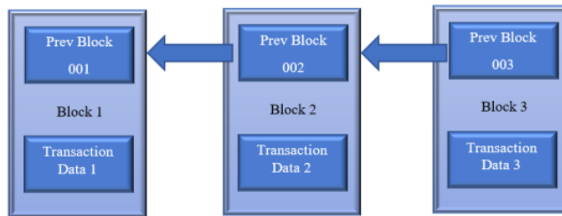
Figure 1. Blockchain Scheme
