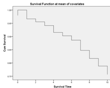
Figure 5. Survival function
