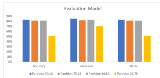
Figure 3. Evaluation Model on Each Data Partition
