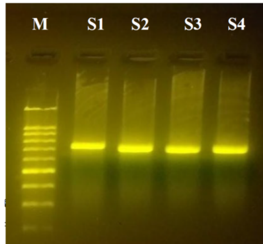
Figure 1. Agarose gel electrophoresis for CYP2C9 gene on 713 bp
