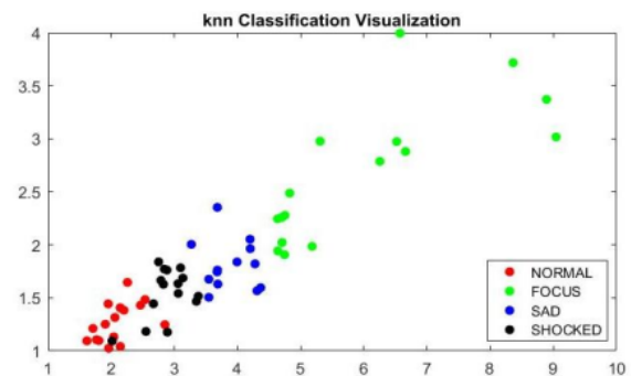
Figure 12: Visualization of KNN classification
