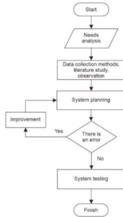
Figure 3. Research Flowchart
