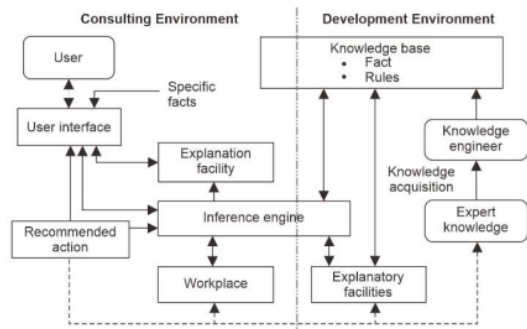
Figure 1. Expert System Architecture.
