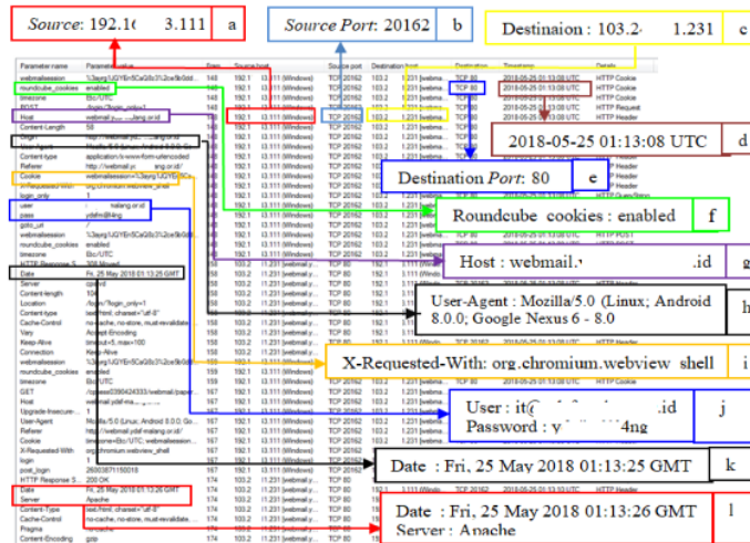
Figure 9. Networkminer sniffing result
