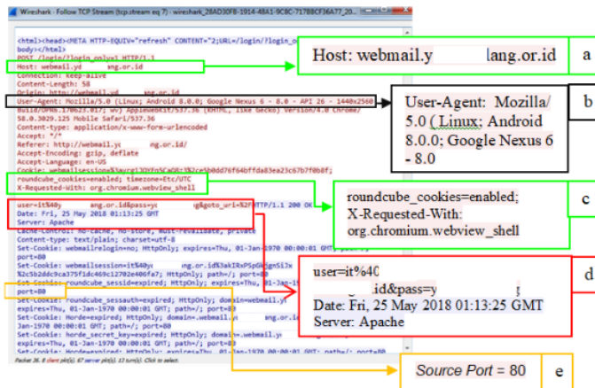
Figure 8. TCP-Stream Wireshark
