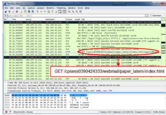
Figure 5. Process examination tools Wireshark
