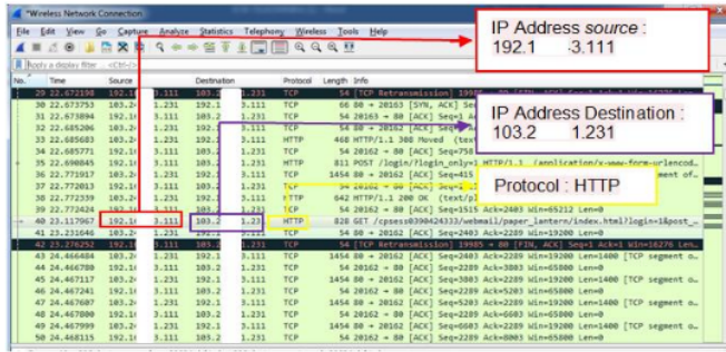
Figure 7. Results of Wireshark sniffing
