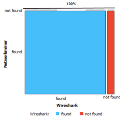
Figure 10. Comparison of forensics tools
