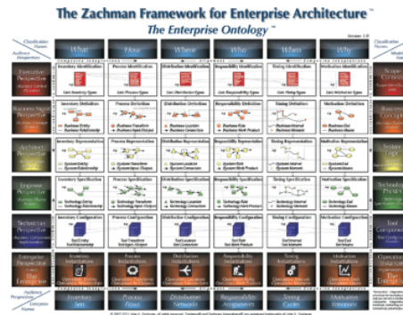
Gambar 2. Zachman Framework
