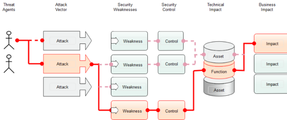
Fig. 2.Application Security Risks
