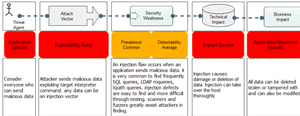
Fig. 4. Vulnerability to injection attacks
