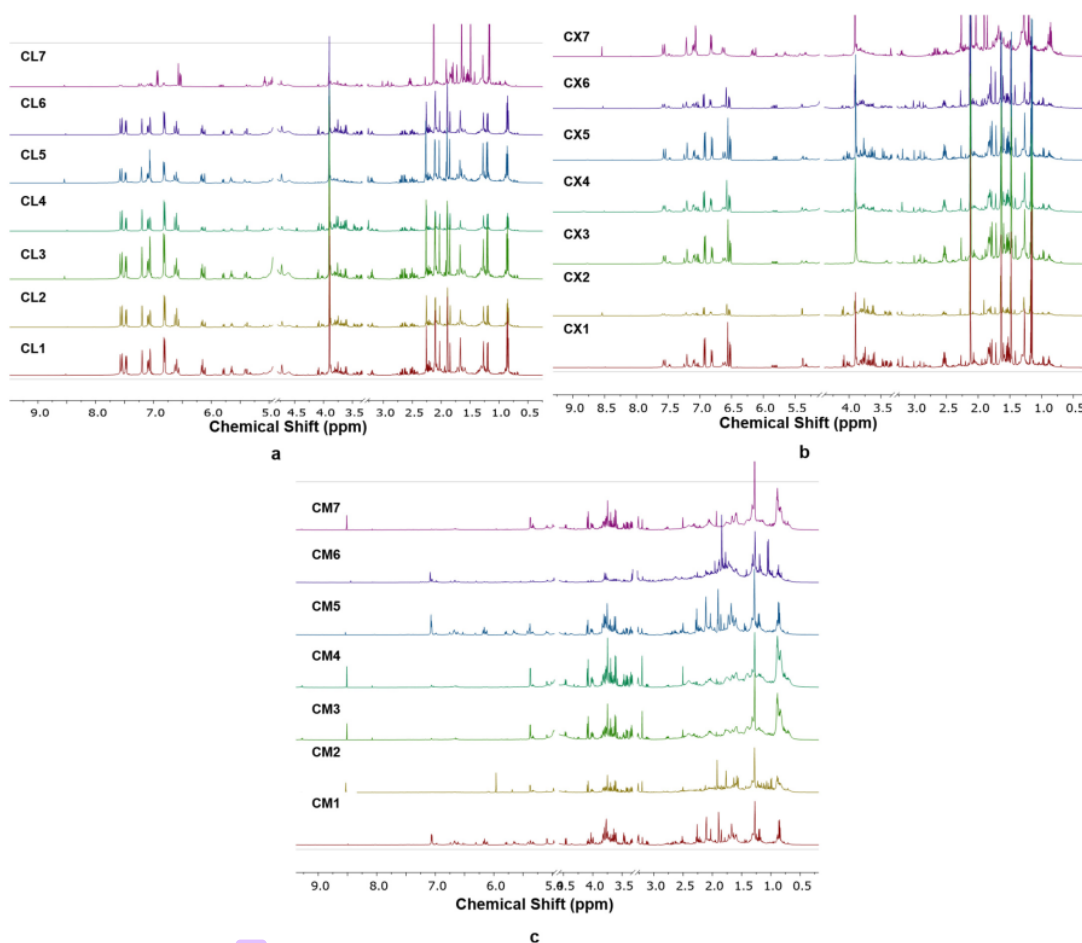
15 Figure 1. ^1\text{H-NMR} spectra of C. longa (a), C. xanthorrhiza (b), and C. manga (c) from different origins.
