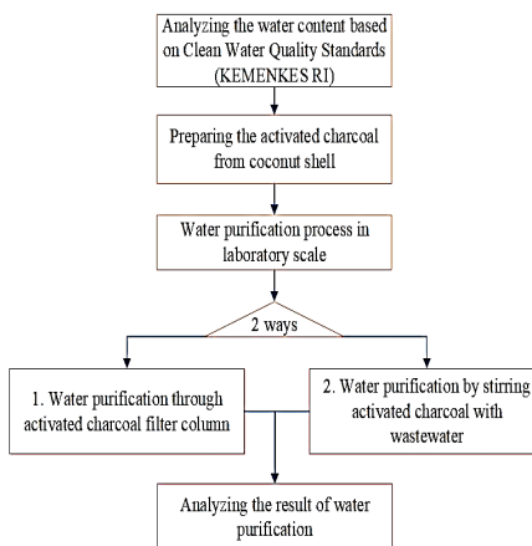
Fig. 1. The stages of water purification
