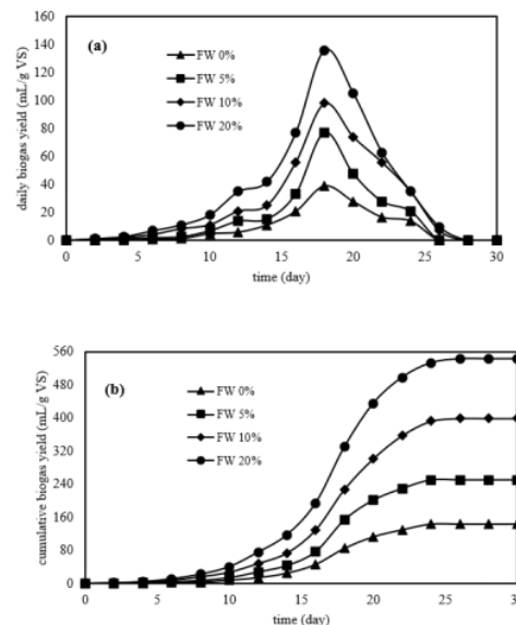
6 Figure 3. Biogas Yields at Different Food-waste Percentage (TS Content = 22%): (a) Daily Biogas Yield, (b) Cumulative Biogas Yield
