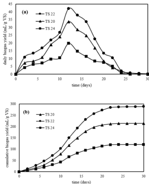
4 Figure 2. Biogas Yields at the Variation of TS Content: (a) Daily Biogas Yield; (b) Cumulative Biogas Yield
