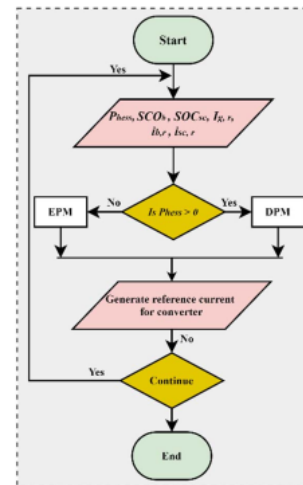
FIGURE 16. Flowchart of the unified HESS controller.
