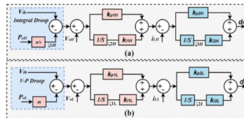
FIGURE 10. Control scheme: (a) integral droop dan double PI controller, (b) traditional V-P droop dan double PI controller.
