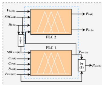
FIGURE 14. FLC-based EMS control scheme.
