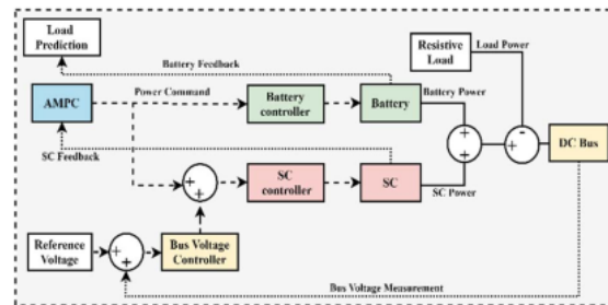
FIGURE 12. Real-time model predictive control scheme.
