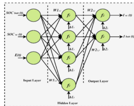
FIGURE 13. Multi-layer feed-forward neural network architecture.
