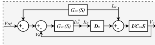
FIGURE 9. Extended droop control scheme.
