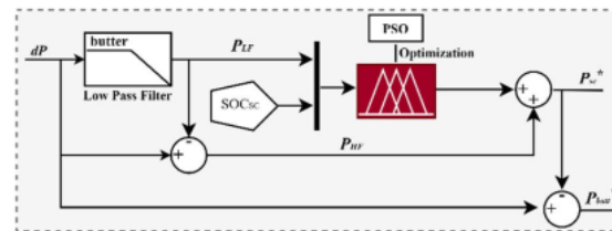
FIGURE 15. Optimized FLC controller scheme with PSO.
