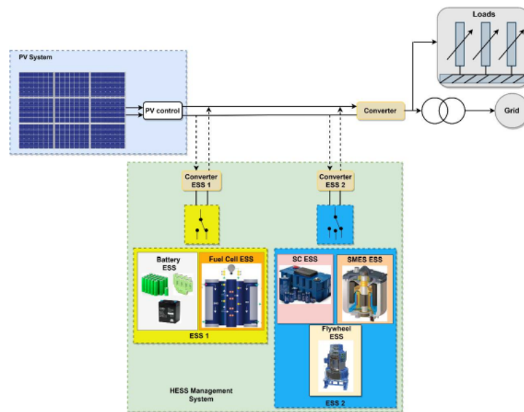
FIGURE 3. The configuration of active parallel HESS topology.
