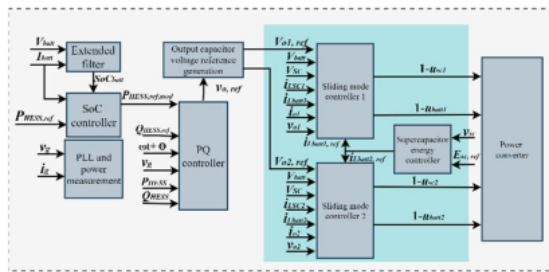
FIGURE 11. Control scheme of the sliding mode (SM).
