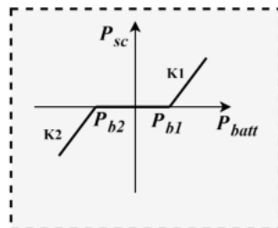
FIGURE 6. RBC control strategy with HESS [129].
