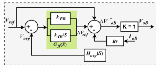
FIGURE 8. Secondary voltage controller scheme.
