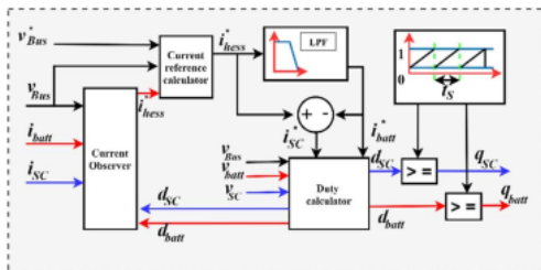
FIGURE 7. Deadbeat control strategy.
