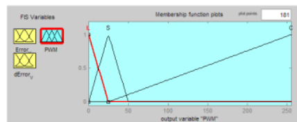
Figure 6. Membership Function of PWM
