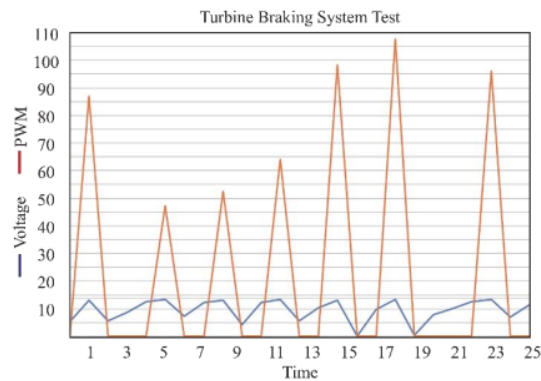
Figure 9. The Test Resulting of The Automatic Braking Proposed Systems
