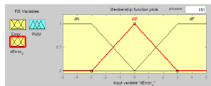
Figure 6. Membership Function of dError_V
