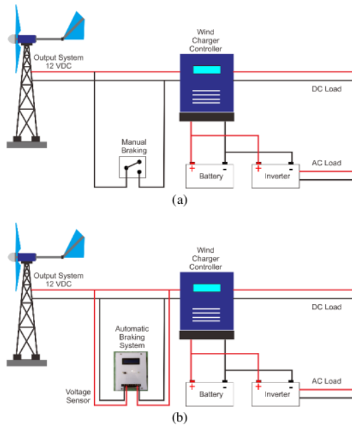
Figure 8. Wind Turbine in PLTH Bayu Baru: (a) Existing System with Manual Braking, and (b) Implementing of the Proposed Systems
