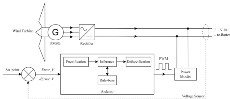
Figure 3. Block Diagram of Proposed Automatic Braking Systems
