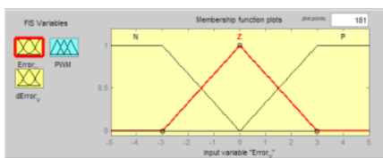
Figure 5. Membership Function of Error_V
