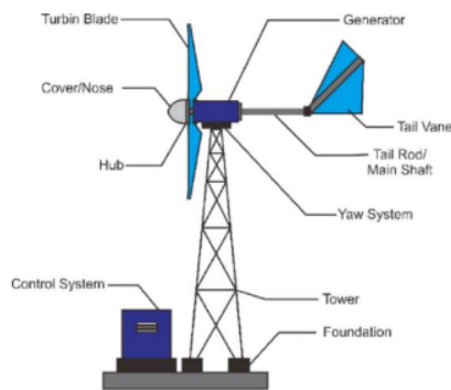
Figure 1. The Construction of Wind Power Plant PLTH Bayu Baru
