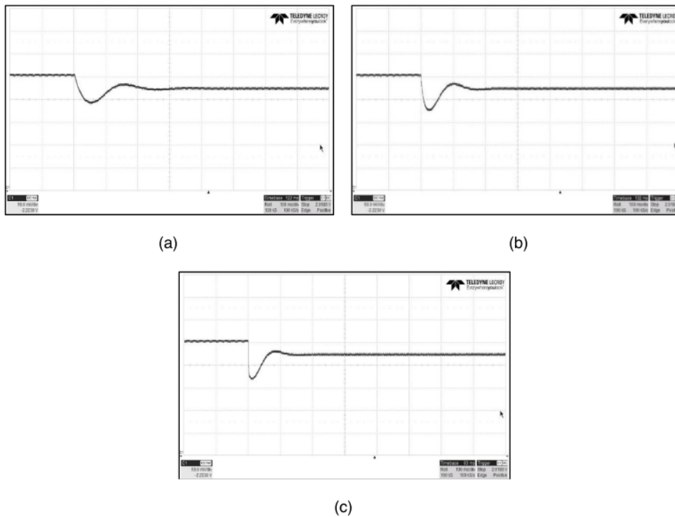
Figure 13. Experimental output waveform for system with different filter cut-off frequencies; (a) 50 rad/s, (b) 100 rad/s (c) 500 rad/s
