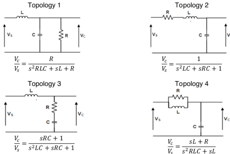
Figure 2. Passive damping topologies
