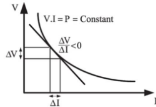
5 Figure 1. Negative impedance characteristic of constant power load
