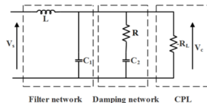
Figure 4. LC filter with passive damping network and constant power load
