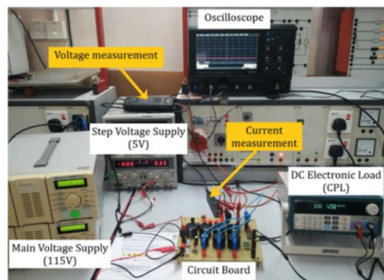
Figure 6. Experimental setup
