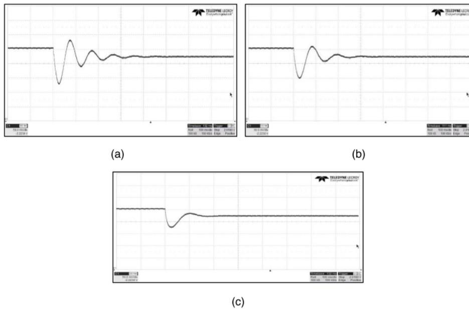
Figure 11. Experimental output waveform for different capacitor relationship with fixed input voltage; (a) C_1 > C_2 , (b) C_1 = C_2 (c) C_1 < C_2
