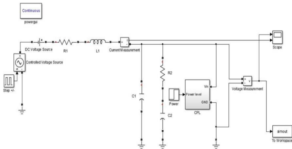
Figure 5. Simulation circuit
