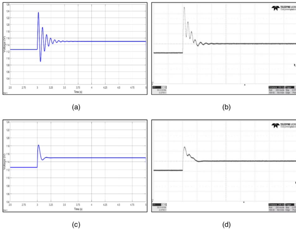
Figure 2. Bus voltage behaviour at 100 W CPL disconnection; (a) simulation without passive damper, (b) experiment without passive damper (c) simulation with passive damper (d) experiment with passive damper
