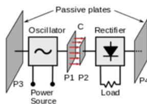
Figure 2. The concept of electrostatic induction
