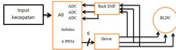
Gambar 3. Diagram blok Back EMF
