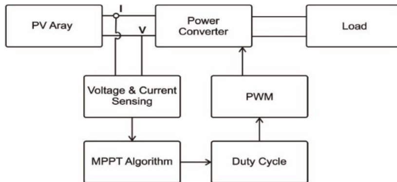
Figure 2. MPPT control strategy.
