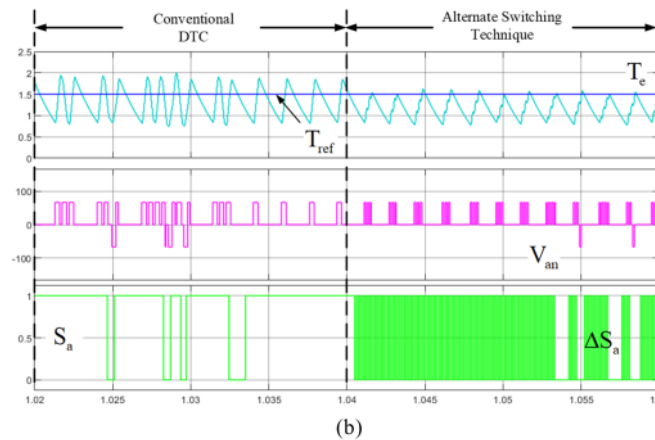
Figure 6. The performance of torque, phase voltage and inverter switching status under hysteresis band size 0.5 Nm. (a) Full scale (b) Magnified scale
