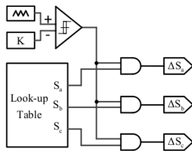
Figure 2. Proposed Alternate Switching Technique
