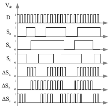
Figure 3. Alternated DTC switching signals
