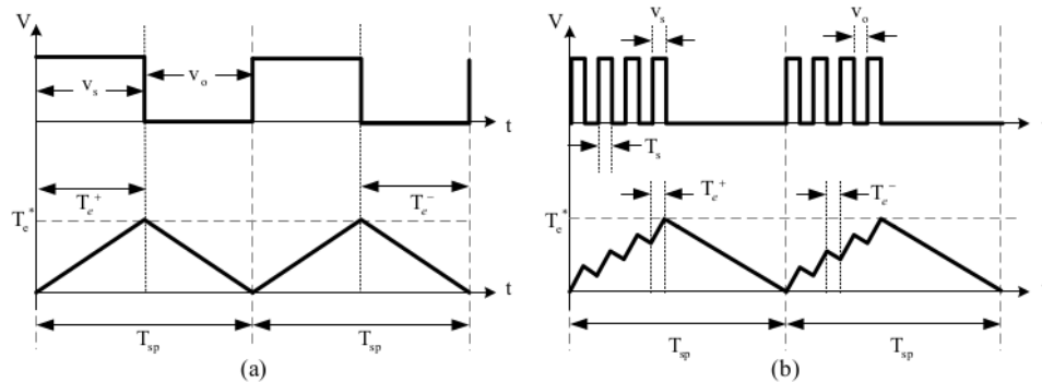
Figure 4. (a) Torque slope condition for conventional DTC scheme (b) Torque slope condition for proposed DTC scheme
