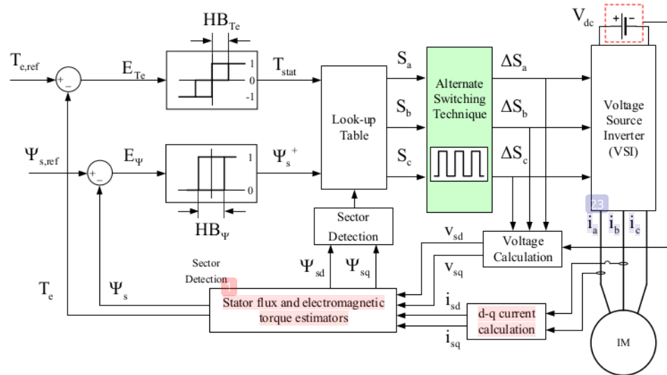
Figure 1. Proposed System with Alternate Switching Technique
