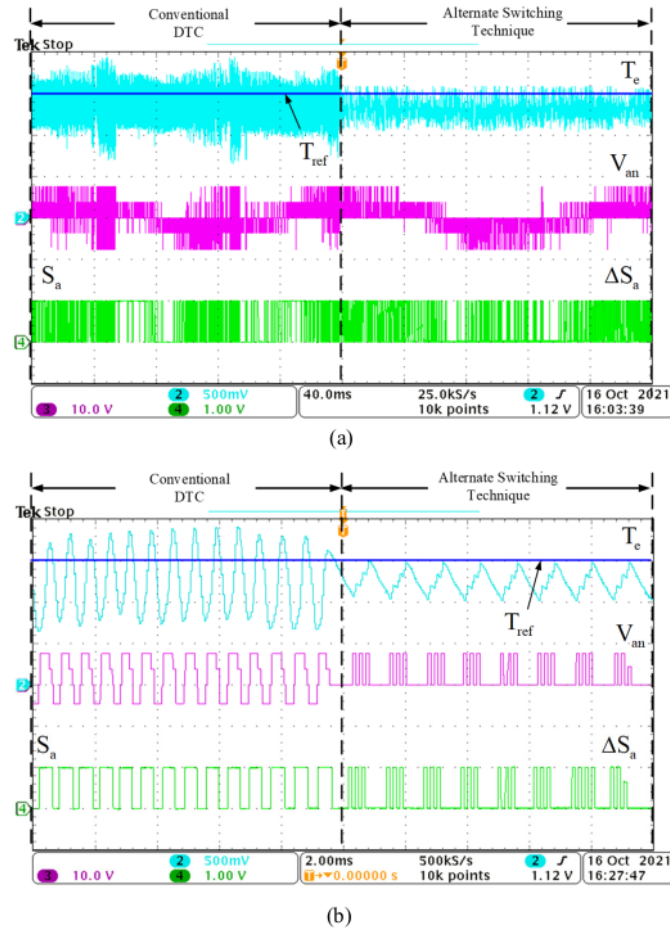
Figure 10. The performance of torque, phase voltage and inverter switching status under hysteresis band size 0.25 Nm. (a) Full scale (b) Magnified scale
