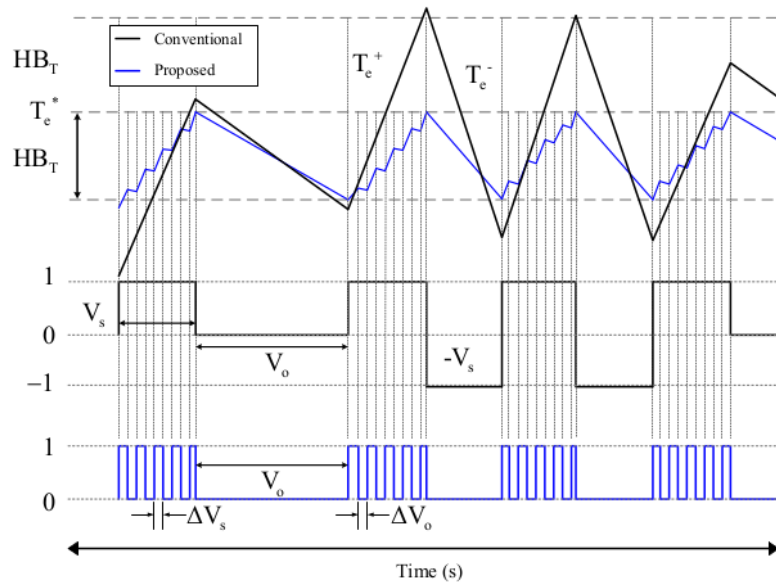
Figure 5. The comparison between conventional DTC and proposed DTC using alternate switching technique
