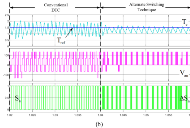
Figure 7. The performance of torque, phase voltage and inverter switching status under hysteresis band size 0.25 Nm. (a) Full scale (b) Magnified scale
