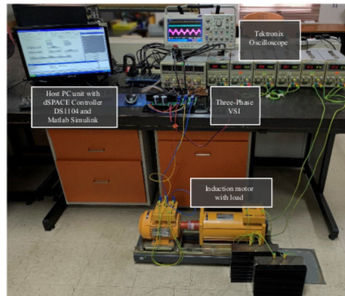
Figure 8. Experimental Setup of DTC drive system
