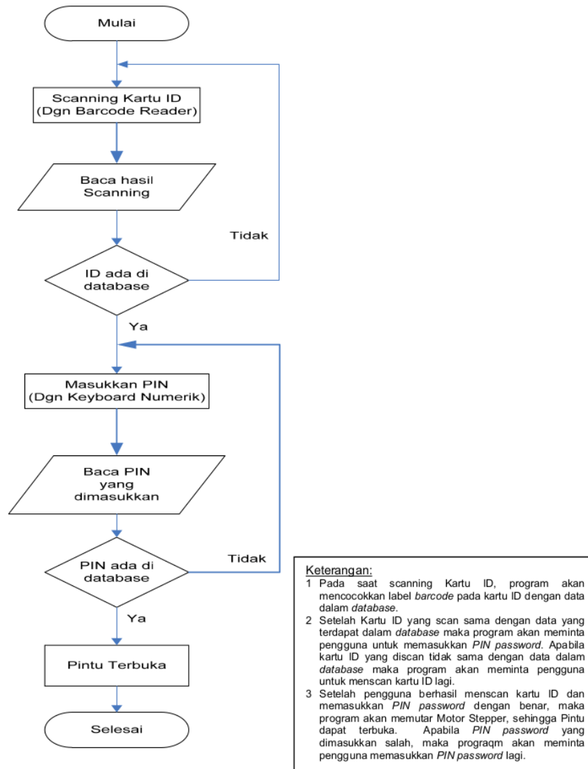
Gambar 1. Flowchart program
