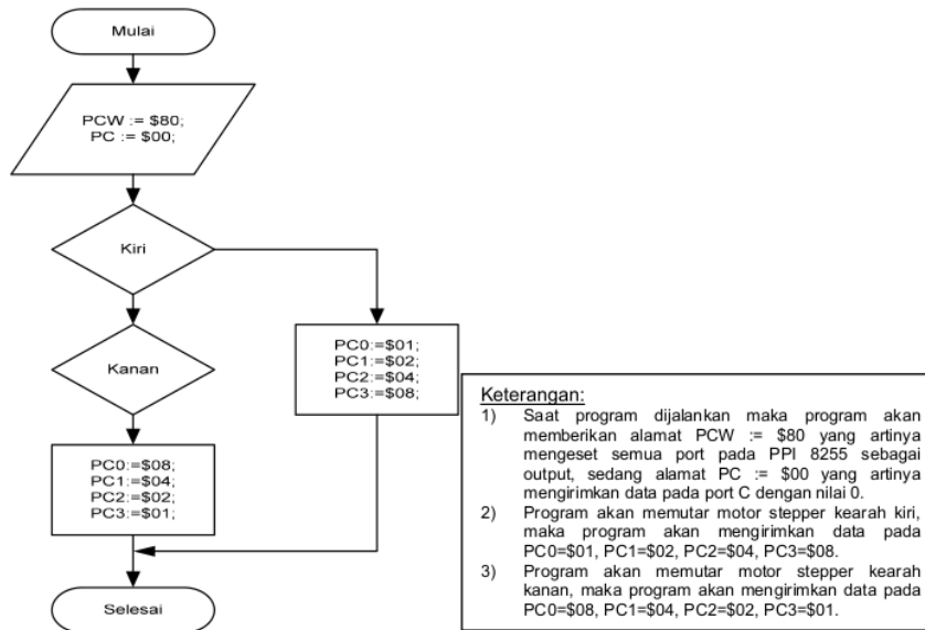
Gambar 2. Flowchart penggerak motor stepper
