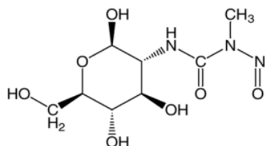
Figure 3. chemical structure of streptozotocin [19].
