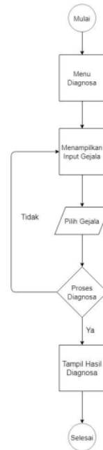
Gambar 1. Flowchart sistem
