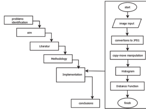
Fig. 5. Research flow chart.
