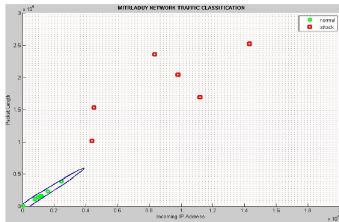
Figure 8. Result of classification in Matlab facility
