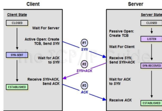
Figure 2. Three way handshake
