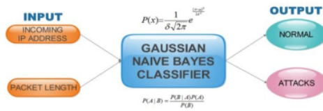
Figure 5. Classification process
