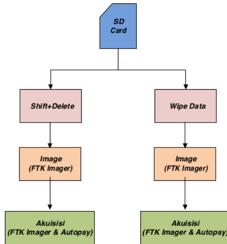
Gambar 4. Tahapan Proses Forensik SD Card
