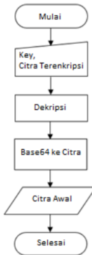
Gambar 4 Diagram Alir Proses Dekripsi
