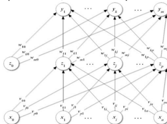
Figure 4. Backpropagation Architecture
