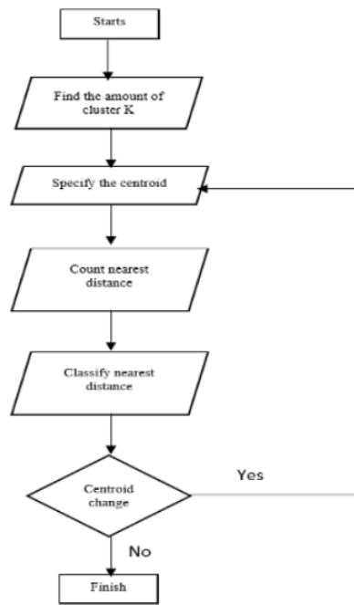
Figure 3. Flowchart algorithm of the K-Means method
