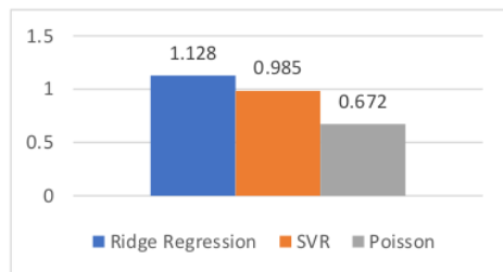
Gambar 6: Grafik Perbandingan Performa RMSE
