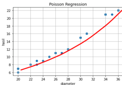
Gambar 2: Hasil Poisson Regression
