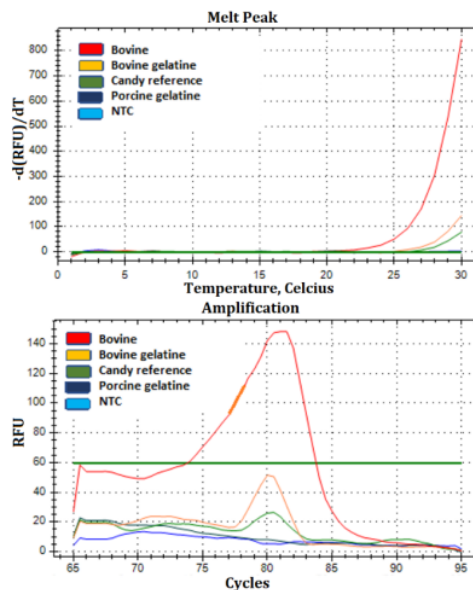
Figure 3. The Amplification Curves during the evaluation of Primer Specificity Test Against Gelatin, Reference and Control Candy (NTC) Using Real-Time PCR.
