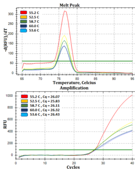
Figure 1. Amplification of designed primers of Primer using different annealing temperature (Ta) to Bovine DNA using Real-Time PCR.
