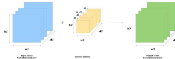
Gambar 3. Convolution layer
