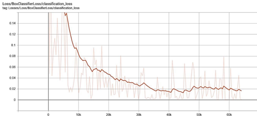
Figure 9. Performance Classification Loss of Faster R-CNN
