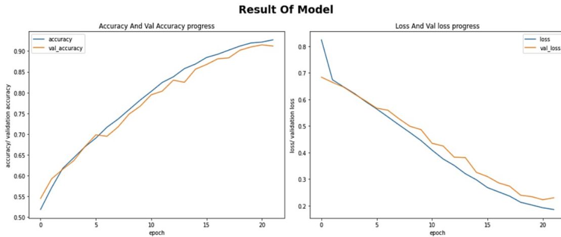
Figure 7. CNN Model System Performance
