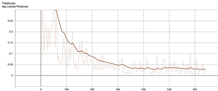
Figure 8. Total Loss System Performance of Faster R-CNN
