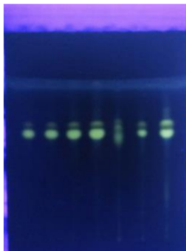
Figure 3. HPTLC profile of berberine standard reference, water and yellow root brackish water decoction on Silica F 254 and elution with the upper phase of n -butanol-acetic acid-water (4:1:5 v/v). HPTLC - densitometry analysis showed that There is no significant different on berberin contents of the water and brackish water decoction so the different effects are not directly corelated to berberine contents. It is possible that there was influence of brackish water on the absorbsion of berberine.
