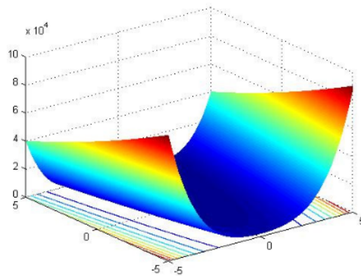
Fig. 3. Rosenbrock's valley function
