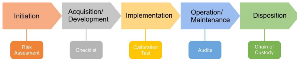
Figure 3. NFLDC Framework
