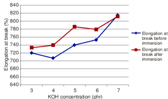
Fig. 7. Elongation at break changes before and after immersion in alkaline at various KOH content
