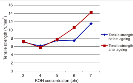
Fig. 2. Tensile strength changes before and after ageing at various KOH content
