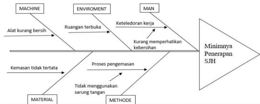
Gambar 1. Diagram Fishbone
