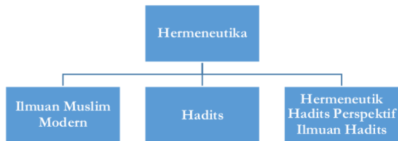
Gambar 1. Alur Penelitian
