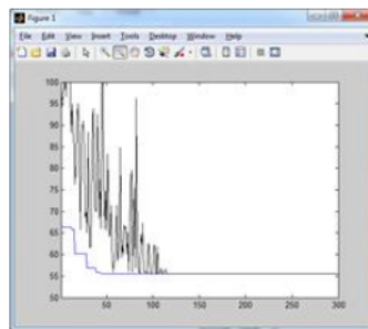
Figure 1.2 Graph Convergence
